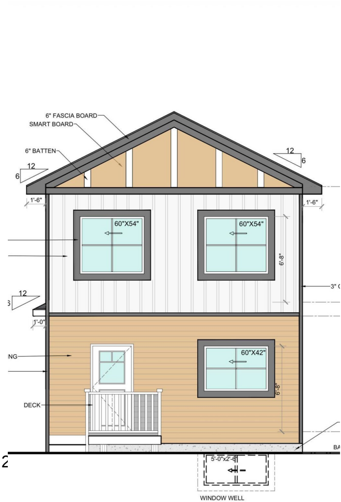
REAR ELEVATION
